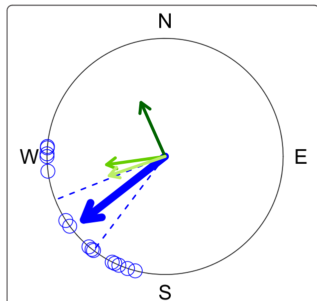
Figure 2 Departure directions of northern wheatears from Wales, Alaska. Departure directions were uniformly distributed towards 233° (Rayleigh test of uniformity: n = 15 , R = 0.87 , P < 0.0001 ; 95% CI: 218° – 249°, range: [205°, 288°]). The blue arrow shows the mean departure direction and its length being a measure of scatter is drawn relative to circle's radius which is one (unit circle). Dashed lines give 95% confidence interval. Equal departure directions were plotted at slightly different directions so that they can be recognized (Table 1). The short arrows indicate the directions of the great circle route (336°, dark green), the constant magnetic course (262°, middle green) and the constant geographic course (251°, light green) from the study site towards Alaskan northern wheatears' wintering area in sub-Saharan Eastern Africa.
